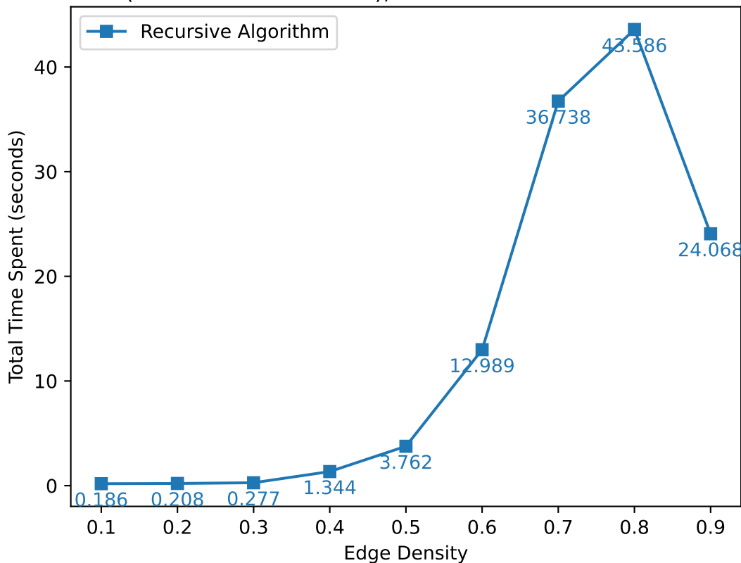
Overall Time Spent on Recursive Algorithm at Different Edge Densities (200 realizations each), basis calculation disabled
